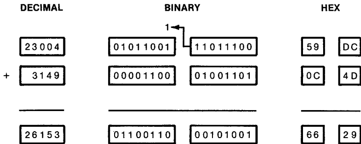
Fig. 12-1. Addition, with carry, of two 16-bit numbers.
